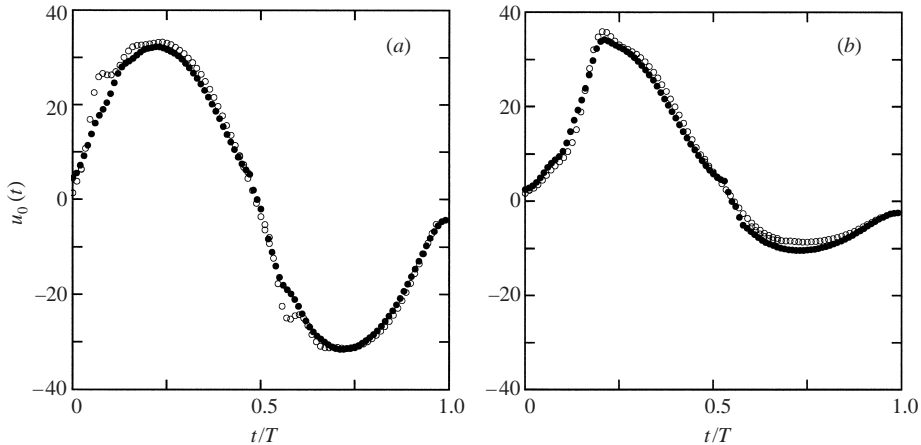
FIGURE 6. Phase locked velocity traces on the centreline of the synthetic jet at (a) x/h = 0 and (b) x/h = 1.5 . \circ , synthetic jet without a step; \bullet , synthetic jet with s/h = 1.5 step.
