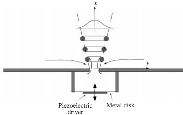
FIGURE 1. Schematic diagram of a synthetic jet.
