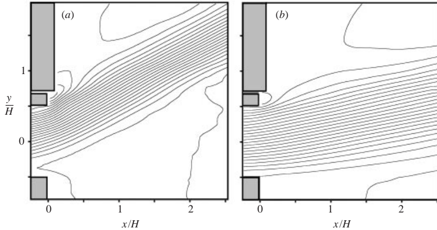
FIGURE 12. Streamline maps of the forced flow for (a) U_{cl} = 7 m s -1 and (b) 17 m s -1 . Contour increments are 5% of the volume flow rate of the unforced flow ( Re_{U_0} = 380 , L_0/h = 19.7 , f = 1120 Hz and s/h = 1.5 ).
